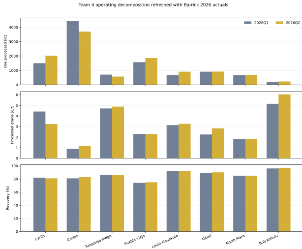
Figure 3. Ore processed, grade and recovery updated with Barrick 2026 actuals. These are physical operating drivers; no commodity-price simulation enters the panel.
