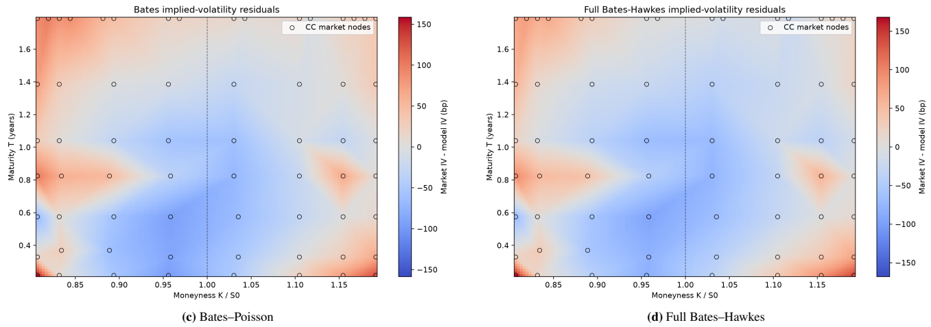
Figure 6. Implied-volatility residual maps for the common 2 September CC64 sample. Blue denotes model IV above market IV and red denotes model IV below market; Heston records the lowest in-sample IV RMSE.
