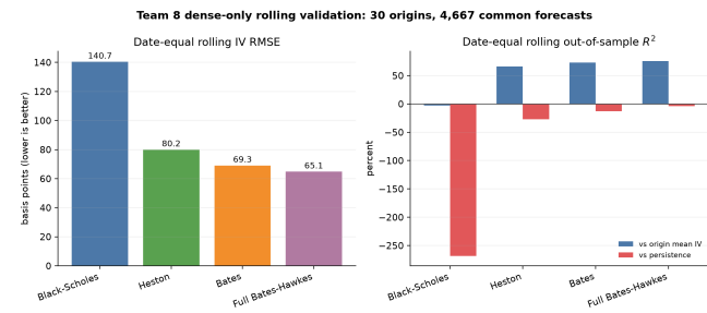
Figure 12. Dense-only rolling evidence on 30 forecast origins and 4,667 common target observations. Full Bates–Hawkes has the lowest date-equal IV RMSE. Positive R^2_{OOS} denotes improvement over the stated benchmark.
